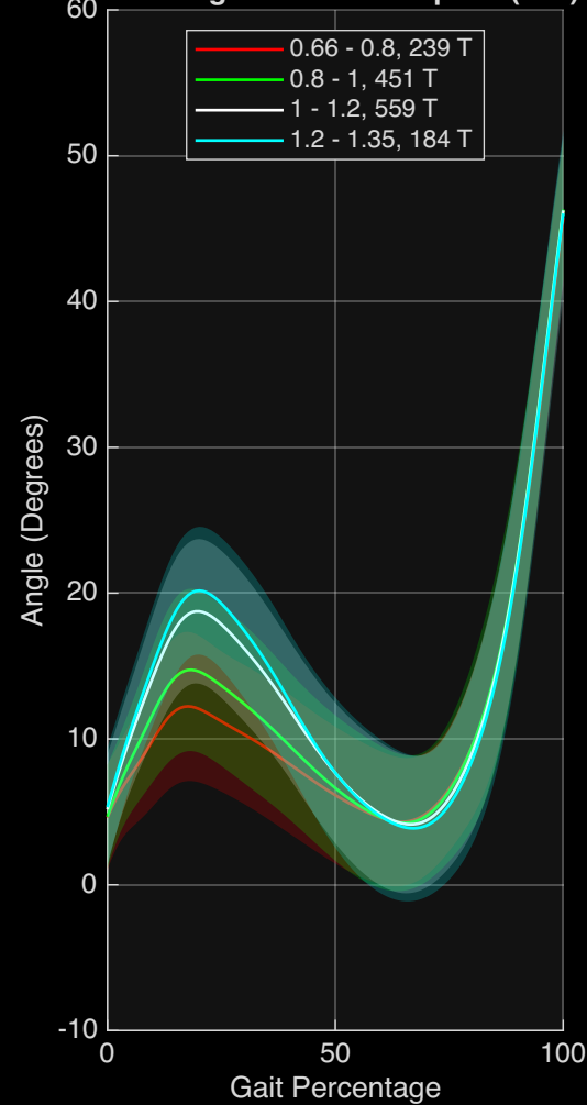
Knee Angle vs Ground Speed (m/s)
